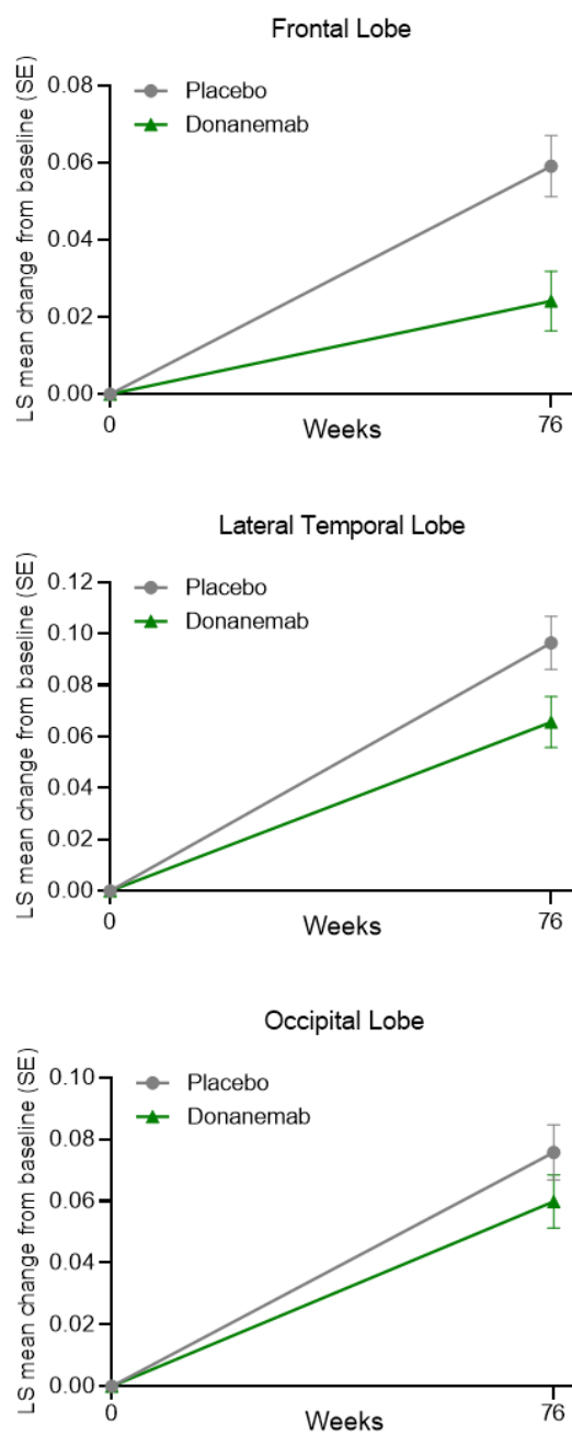
Figure S2. Regional SUVr analyses of tau accumulation with cerebellar gray reference
